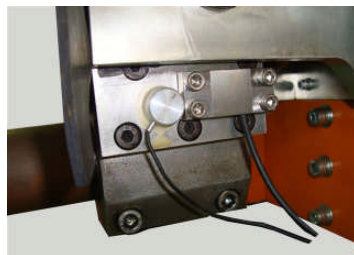
Welding-force Sensor (example)
