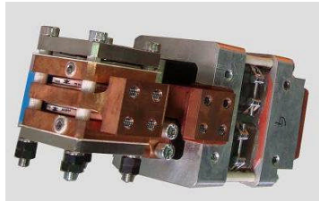
Transformer
